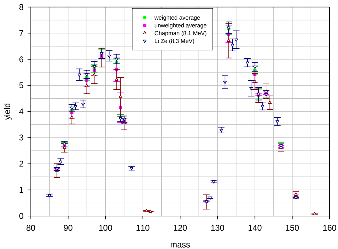
Benchmark A: ^{238}\text{U} at 8.1-8.3 MeV, experimental yields and averages
